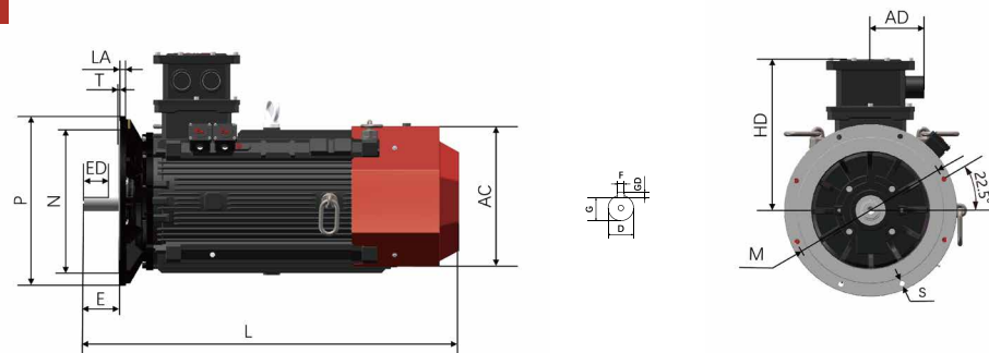
YBX3-315~355
